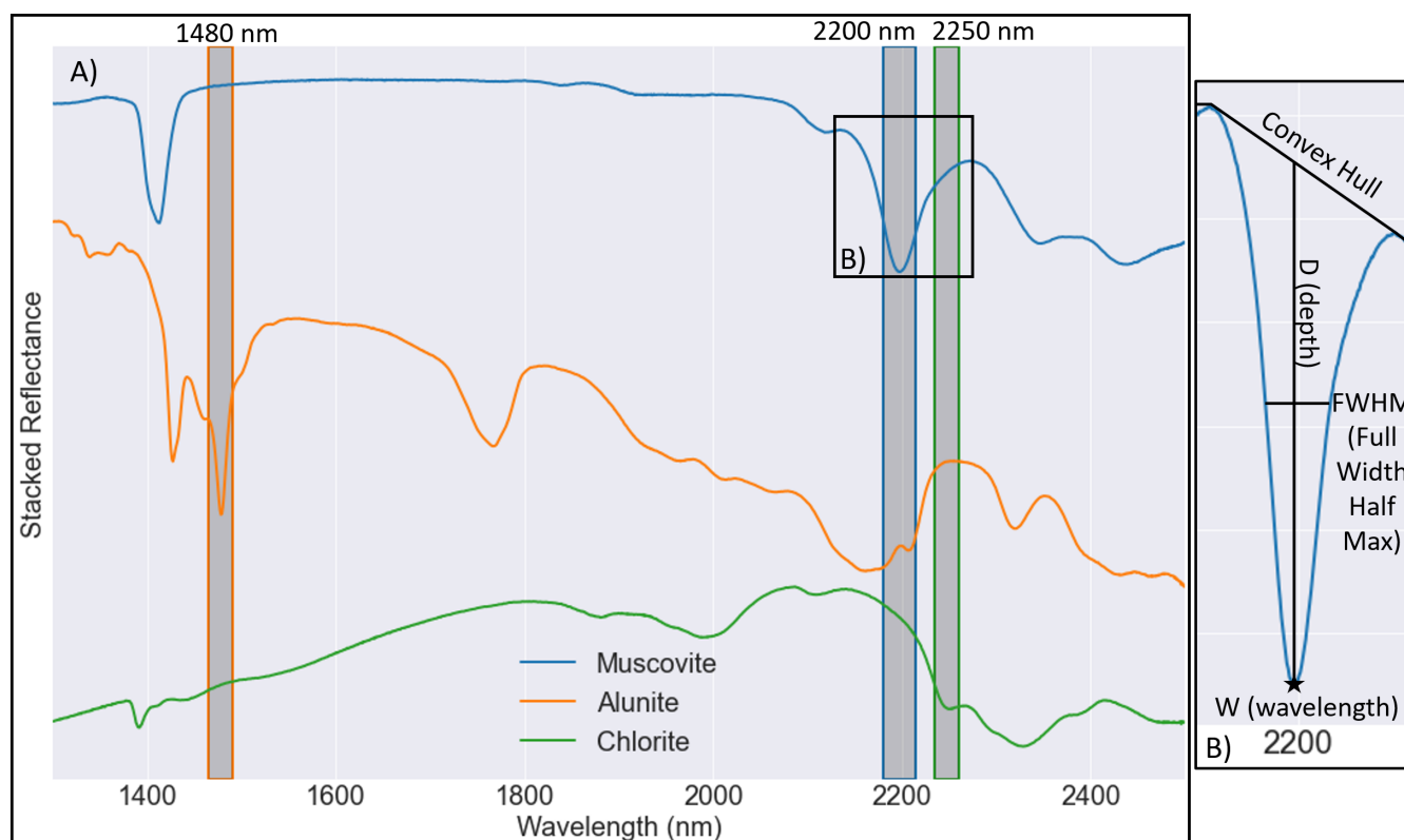
Figure 1. Examples of SWIR spectra extracted from the JPL Ecostress spectral library (Grove et al. 1992), showing key absorptions for the three minerals discussed as vectors. Inset (B) illustrates the nomenclature of absorption feature scalars applied to the 2200nm “AIOH” absorption for muscovite. Depth is measured from the base of the absorption (the minimum) vertically to where it intercepts the convex Hull line, formed by connecting apices along the spectral curve. FWHM is measured at the midpoint of D, between either side of the absorption feature.
